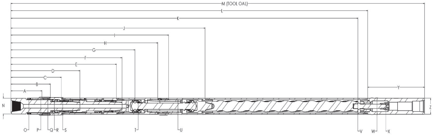
Sealed Bearing Fishing Dimensions
