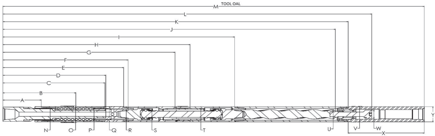
Mud Lube Fishing Dimensions
